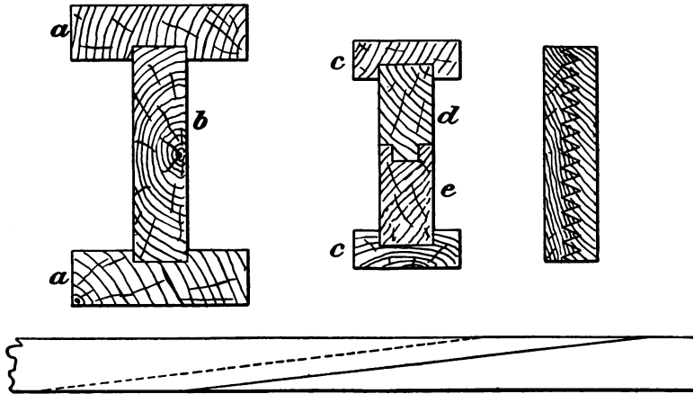
Fig. 45.—System of splicing and building up wooden members. When they have to be curved and to keep their shape, they should be bent at the curve at the time of being glued together, and joined in the middle as at d .
